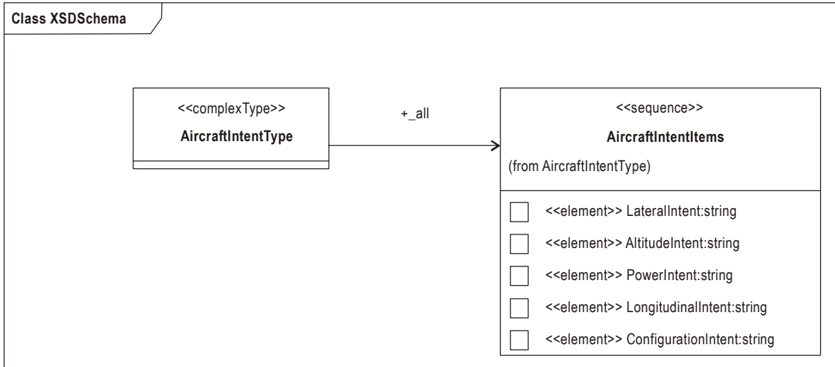
Figure E-5. Aircraft intent XML schema diagram
