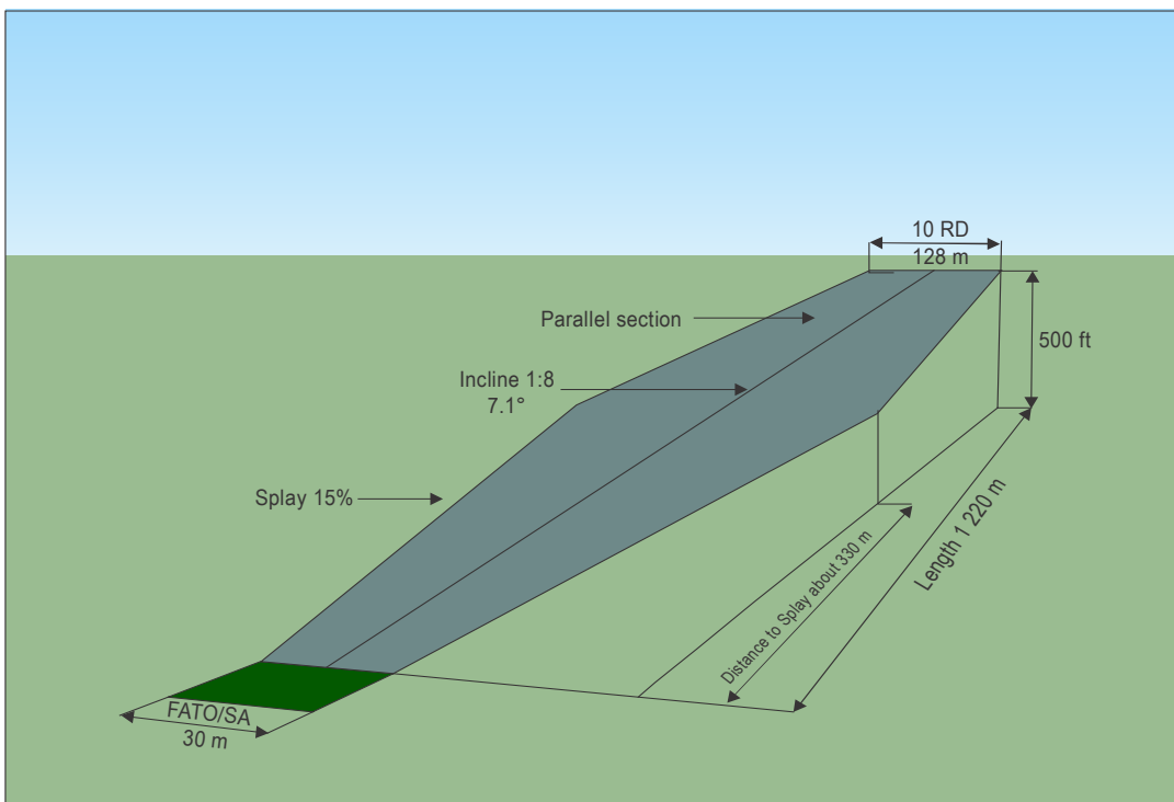
Figure II-4-19. Night Category C slope (15 m D-value)
