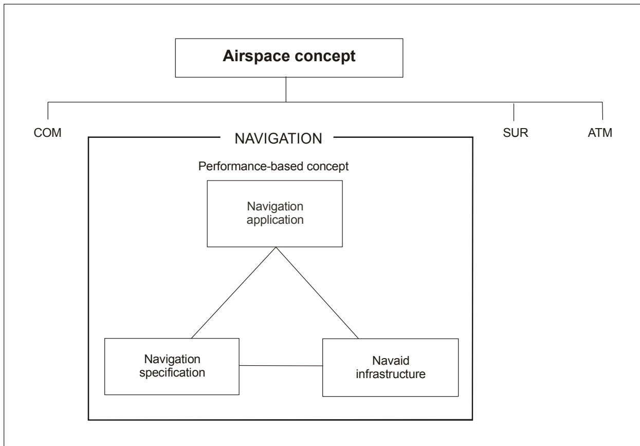
Figure I-A-1-1. PBN concept
