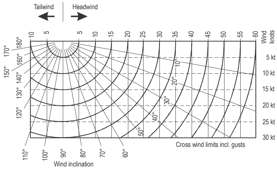
Figure F-5. Typical wind limit diagram
