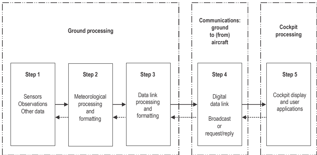
Figure H-1. METLINK system overview
