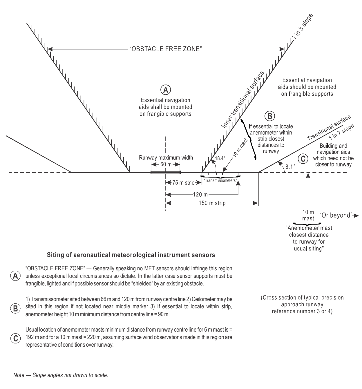
Figure B-2. Obstacle limitation surfaces
