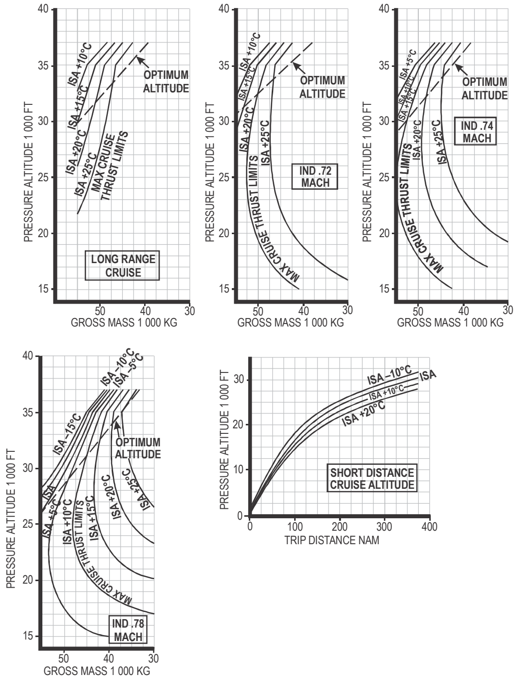
Figure F-3. Optimum flight level (for B737) as a function of take-off mass and temperature deviation from standard
