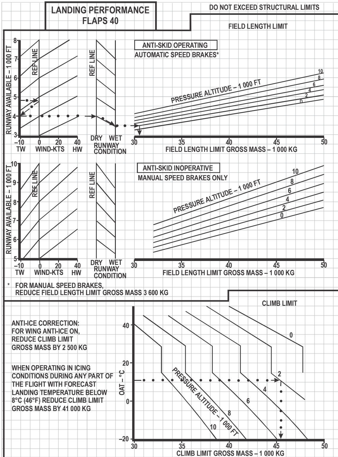
Figure F-6. Landing performance calculations
