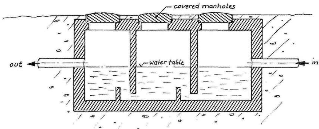
Figure 5-3. Sub-surface fuel separator
