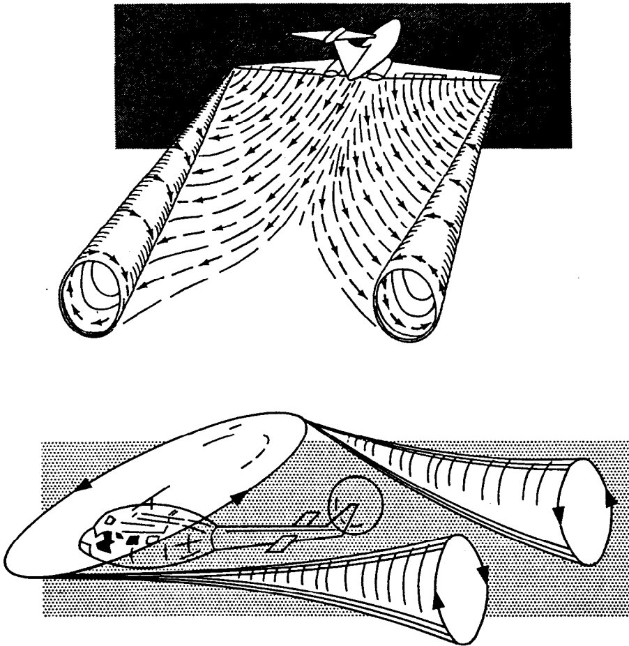
Figure 1.— The rolling-up process
