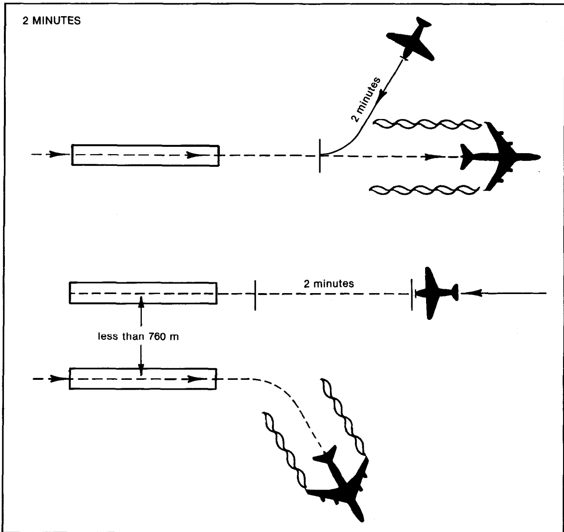
Figure 7.— For opposite-direction aircraft (see 3.2.4.5 b))
