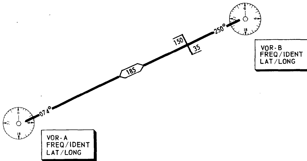
Figure 2. Charting of VOR route segment with off-centre change-over point
