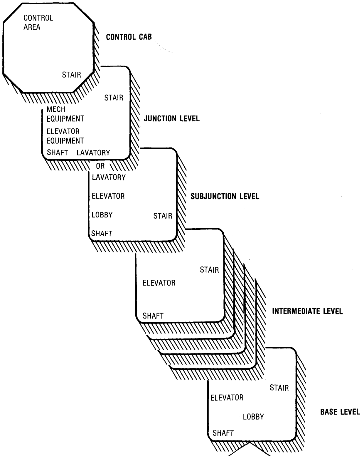
Figure 6.— Diagram of the level arrangement in the non-functional shaft of an aerodrome control tower
