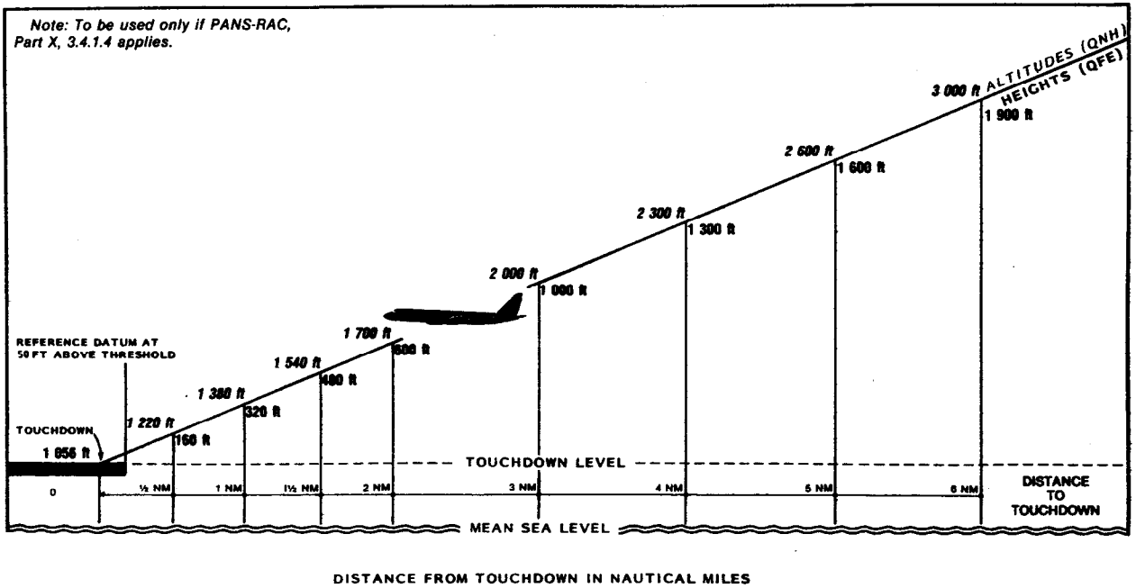
Figure 2 b).— Typical pre-computed levels for a 3-degree glide path — (non-SI alternative units)
