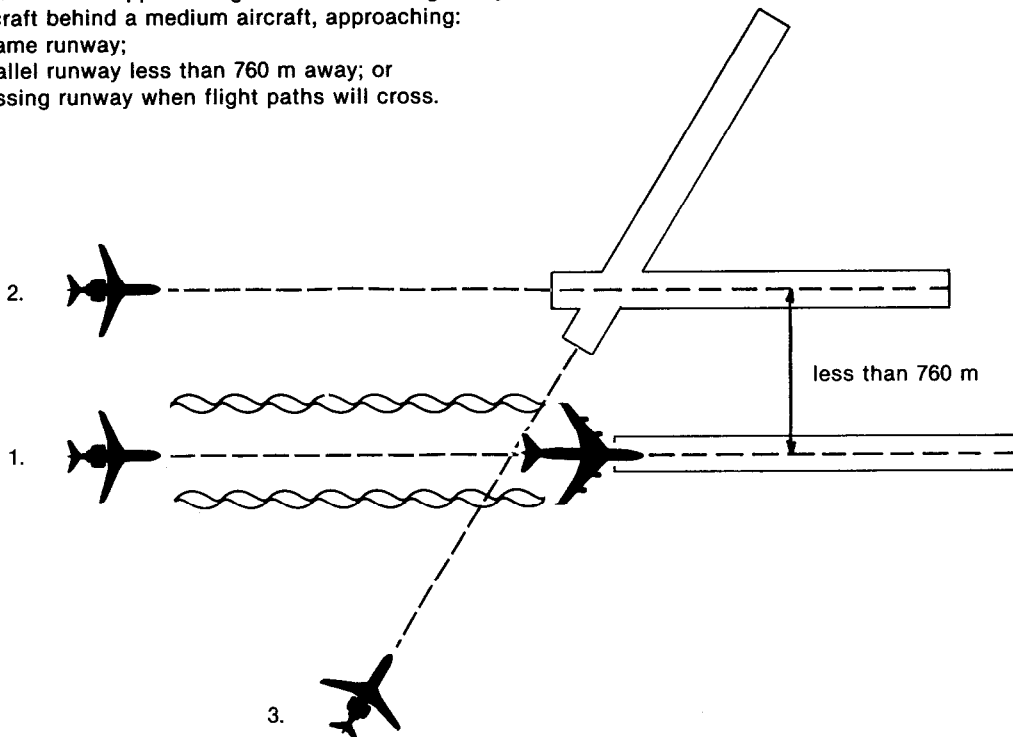
Figure 8.— Cautionaries — Visual flight rules (VFR) and visual approaches (see 3.2.5)
