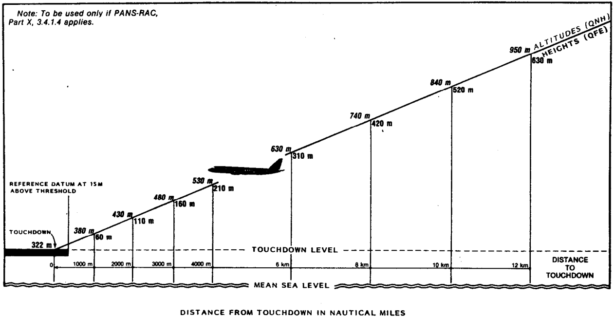
Figure 2 a).— Typical pre-computed levels for a 3-degree glide path — (SI units)
