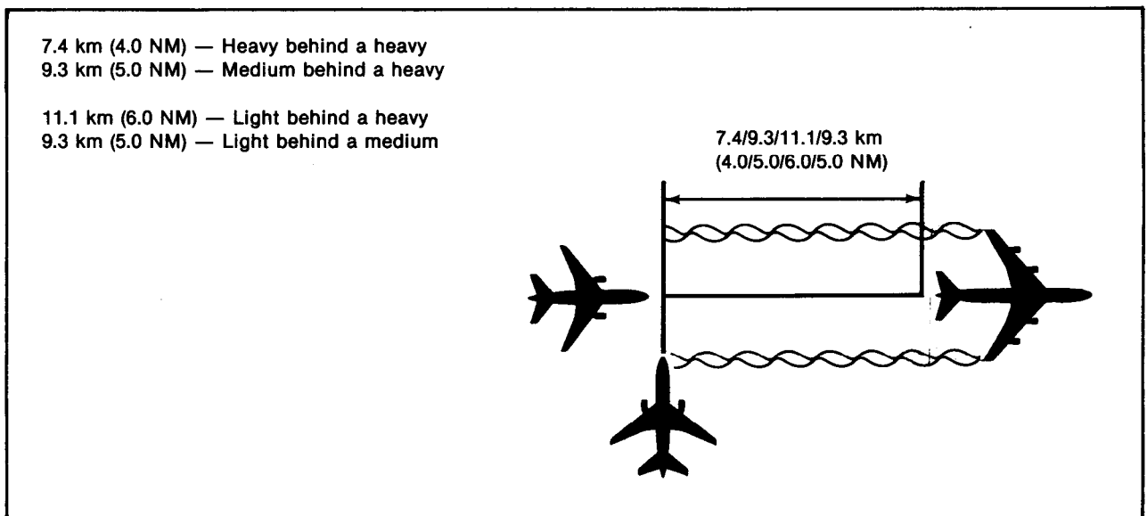
Figure 2.— Wake turbulence separation minima for crossing and following aircraft (see 3.2.4.2)
