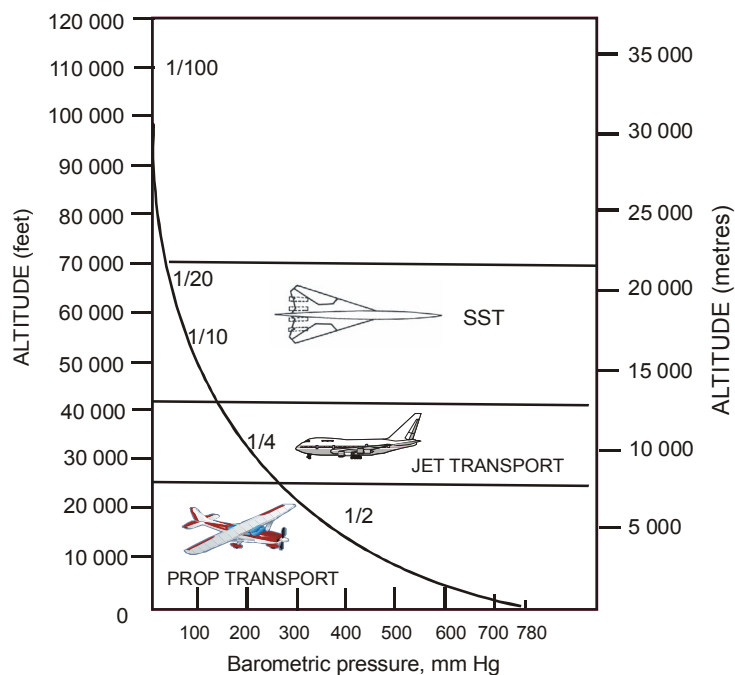
Figure II-1-3. Barometric pressure and altitude
