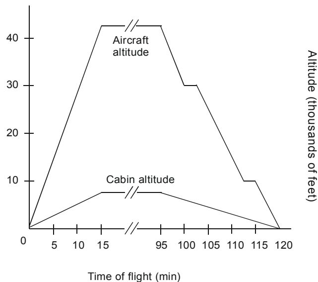
Figure II-1-4. Aircraft and cabin altitudes for a commercial aircraft during a typical flight 1
