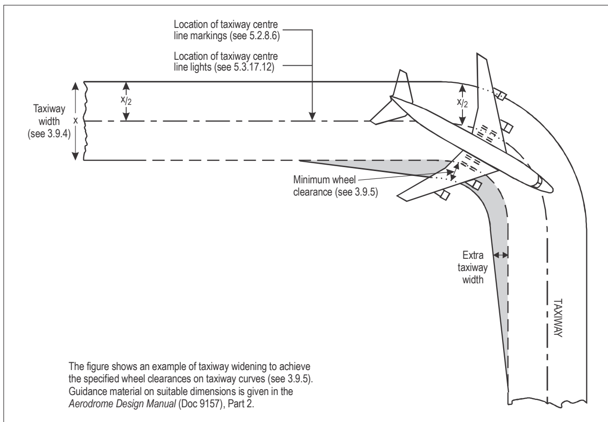
Figure 3-2. Taxiway curve
